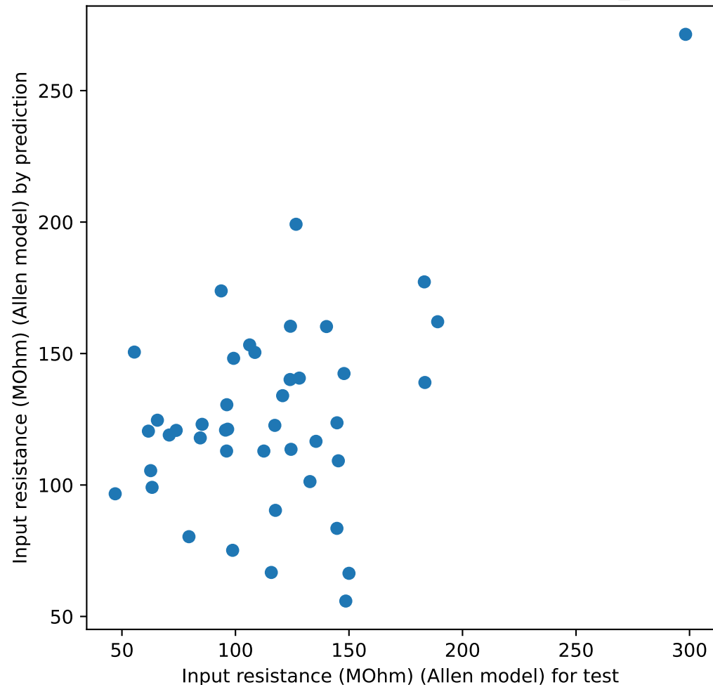
prediction of Input resistance (MOhm) (Allen model) by embs alpha 0.9 l1_ratio 0.0 positive False MAE 36.49
